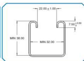
Strut Dimensions
